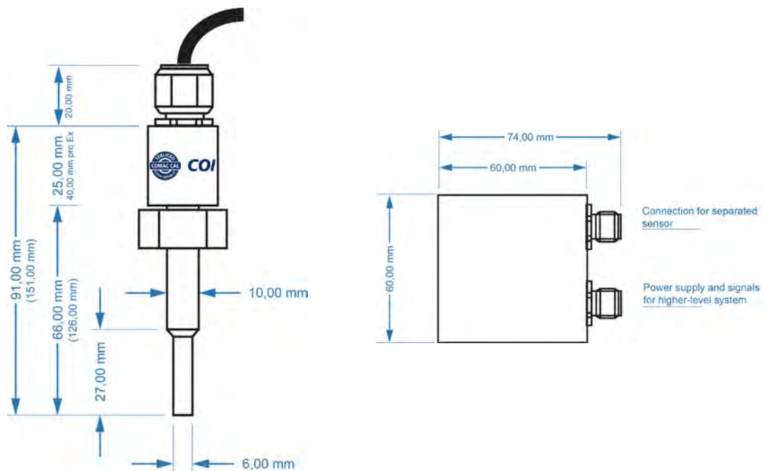
Separate version for DIN rail or wall mounting
