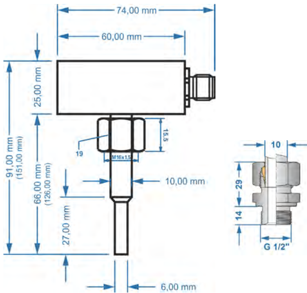
Separate version for DIN rail or wall mounting
